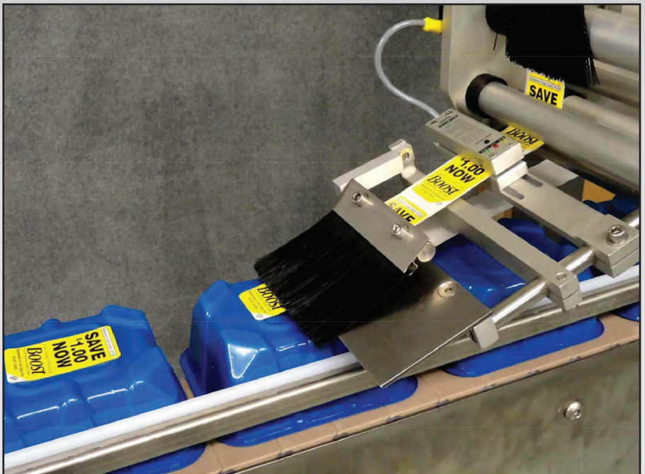
Model CLAS overhead mounted wipe-on applicator
